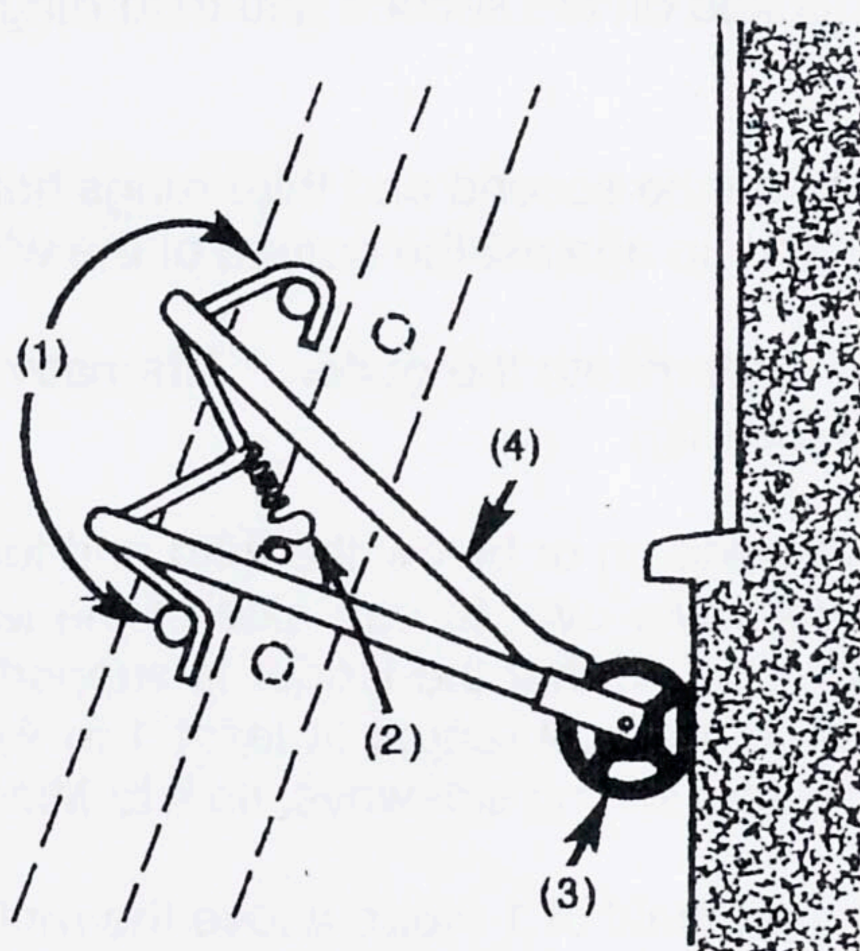
LADDERFIX MICROLITE on walls.
